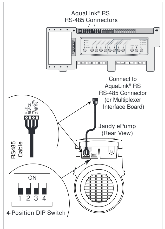
Figure 3. Wiring AquaLink® RS Controller or AquaLink® PDA to ePump
